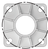
AL-5 Template 11.00 X 11.00 X 1.00 Anchor Plate 11.50-11.75" DIA. Bolt Circle
