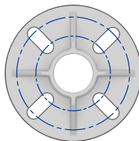
AL-3 Template \varnothing 11" \times 0.75" Anchor Plate 6" - 9" DIA. Bolt Circle
