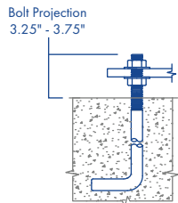
ANCHOR BOLT DETAIL
