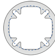
Anchor Plate 10" Diameter 7" B.C.D.
