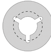
Anchor Plate 6" Diameter 3.5" B.C.D. 2.25" Conduit Opening
