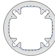
Anchor Plate 11.5" Diameter 8" B.C.D.
