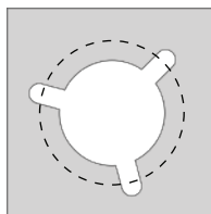
Anchor Plate 8" Square 5.25" B.C.D. 4" Conduit Opening
